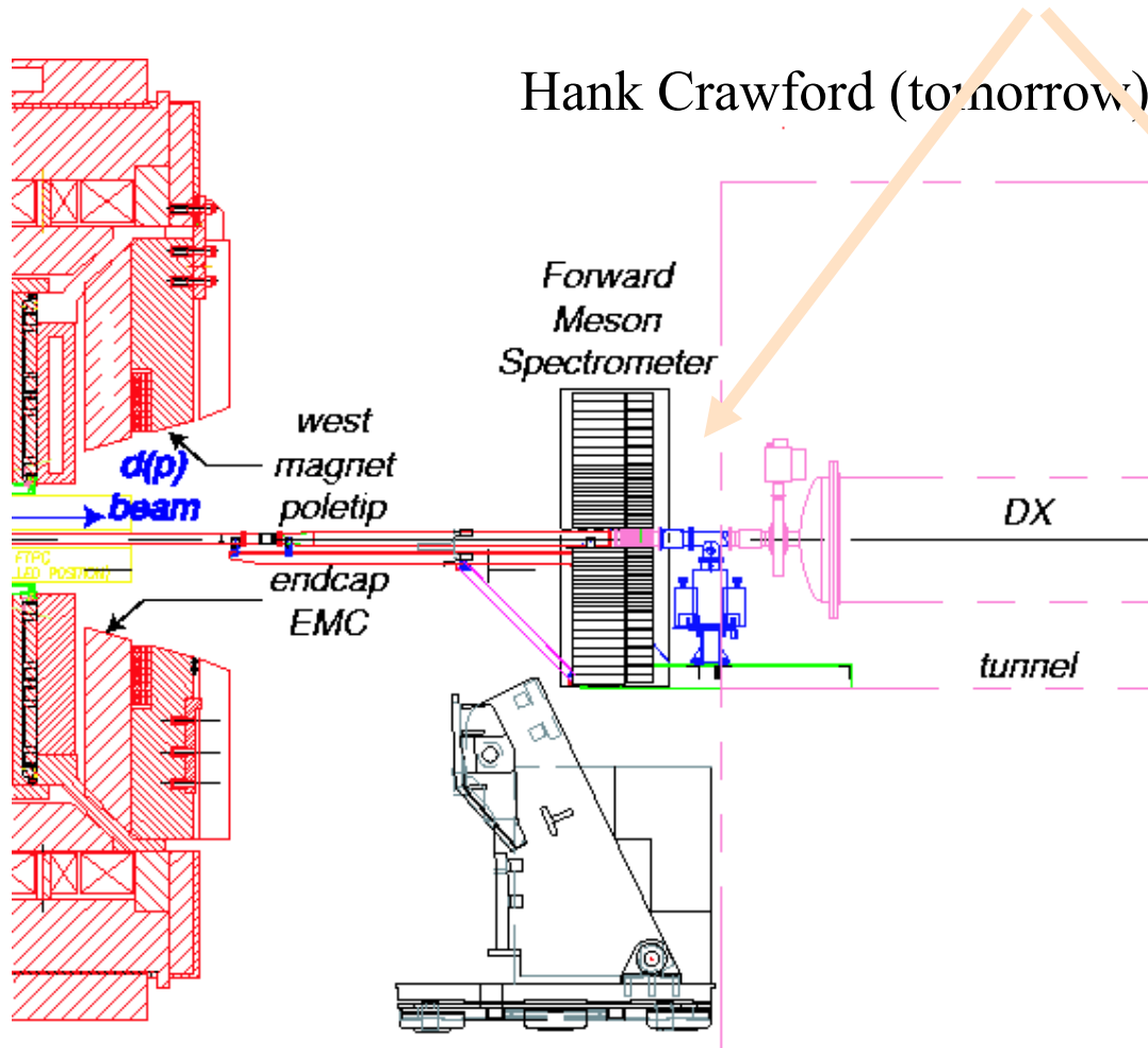
Side View of the West Pole Tip
