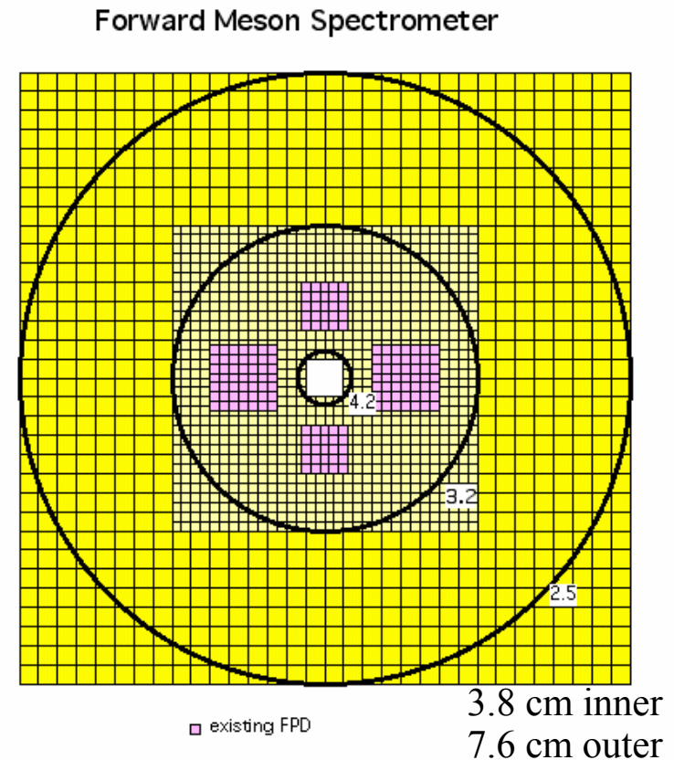
End View of the PbI Array ~ 2.4 m square, ~ 1500 PMTs
