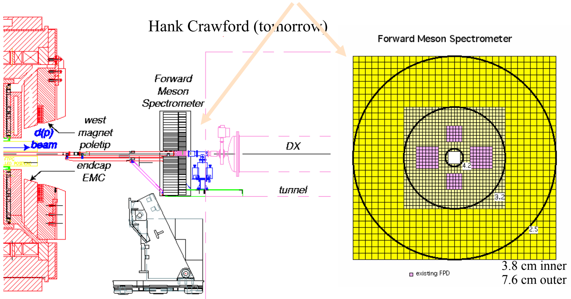
End View of the PbGI Array ~ 2.4 m square, ~ 1500 PMTs
