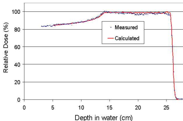
Figure 7, A typical Spread Out Bragg Peak (SOBP)
