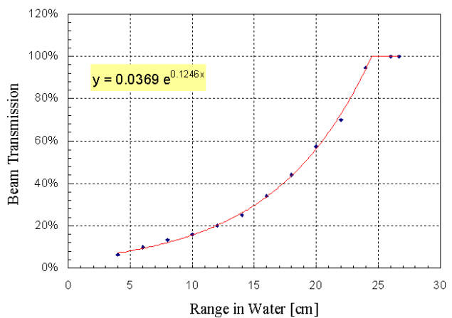
Figure 3, Transmission through ES1 vs. range in water.
