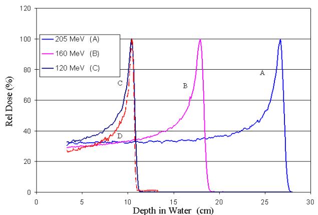
Figure 4. Pristine peak width vs. incident beam energy. Curve D shows the effect of the Momentum band slits.
