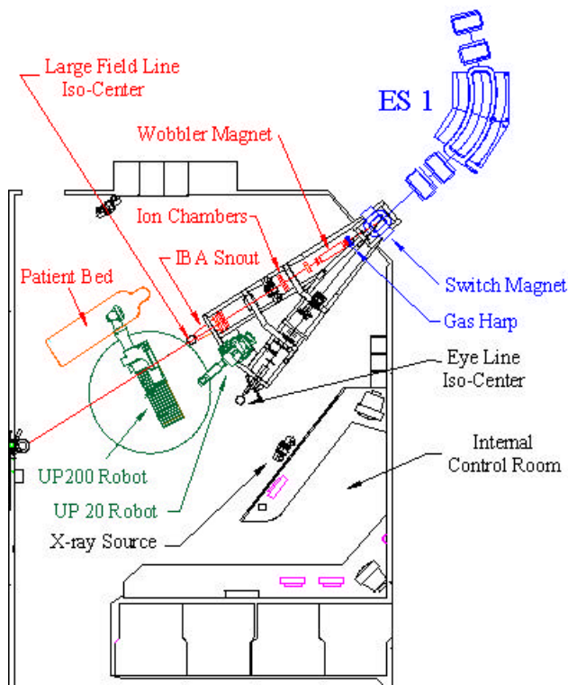
Figure 5. Layout of the fixed horizontal Treatment Room.
